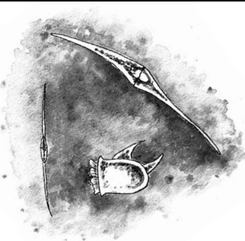
Phytoplankton: Dinoflagellates Ceratum spp., Ceratium fusus , Dinophysis antarctica
